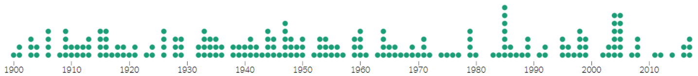
Number of hurricanes that made landfall in the continental United States
